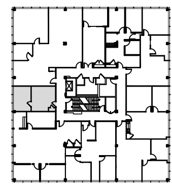
2ND FLOOR KEY PLAN
